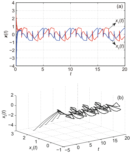
Fig. 6 State trajectories (a) and phase plots (b) of system (19) with \omega = 2 . Reprinted from Li XD and Shen (2010), Copyright 2010, with permission from IEEE
