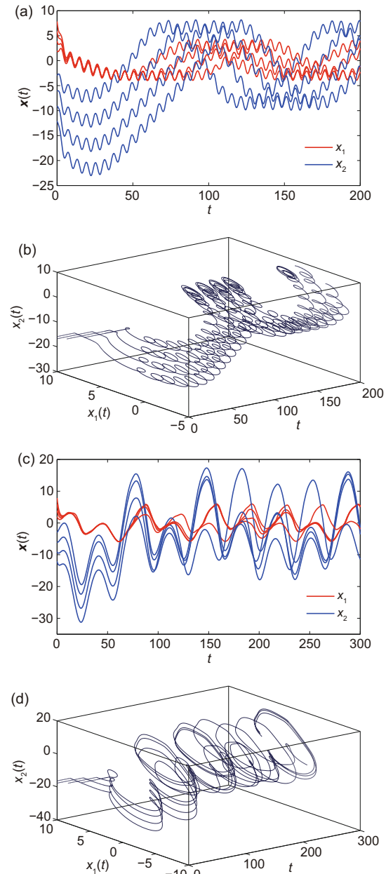
Fig. 4 State trajectories of system (16) with \omega=6 and without impulsive control (a), phase portraits of system (16) with \omega=6 and without impulsive control (b), state trajectories of system (16) with \omega=35 and without impulsive control (c), and phase portraits of system (16) with \omega=35 and without impulsive control (d). Reprinted from Li XD and Song (2013), Copyright 2013, with permission from IEEE
